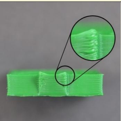
Clogged Extruder
